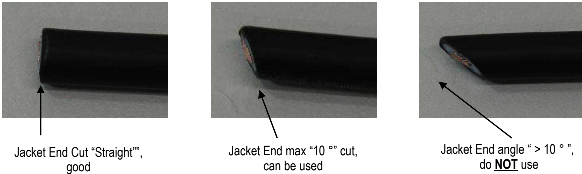
Figure 3.1 Cable cuts
